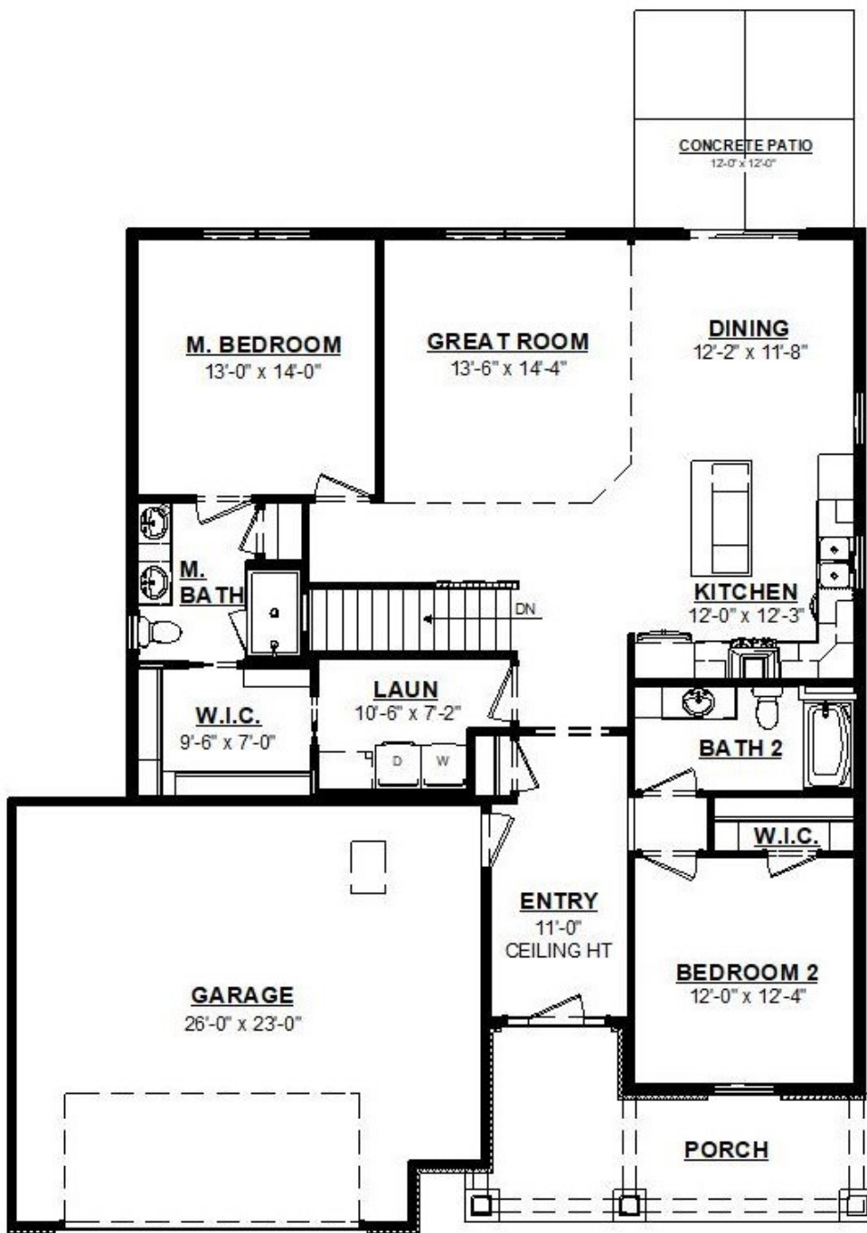
First Floor
